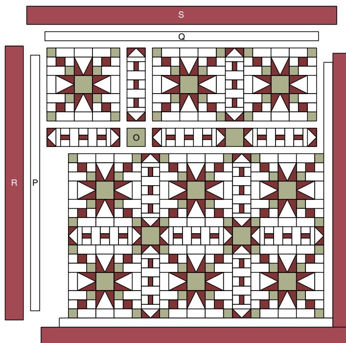
Snow Day Assembly Diagram 68" x 68"
